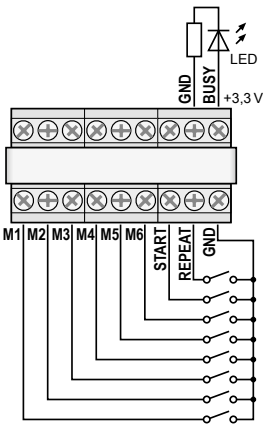
⑤ Connection for remote control
